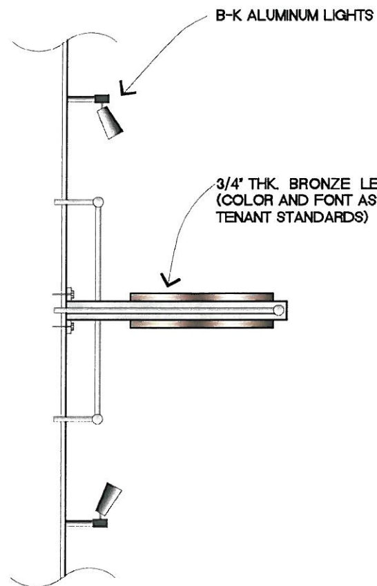
BLADE SIGN TOP VIEW SCALE: 1/2" = 1'-0"
