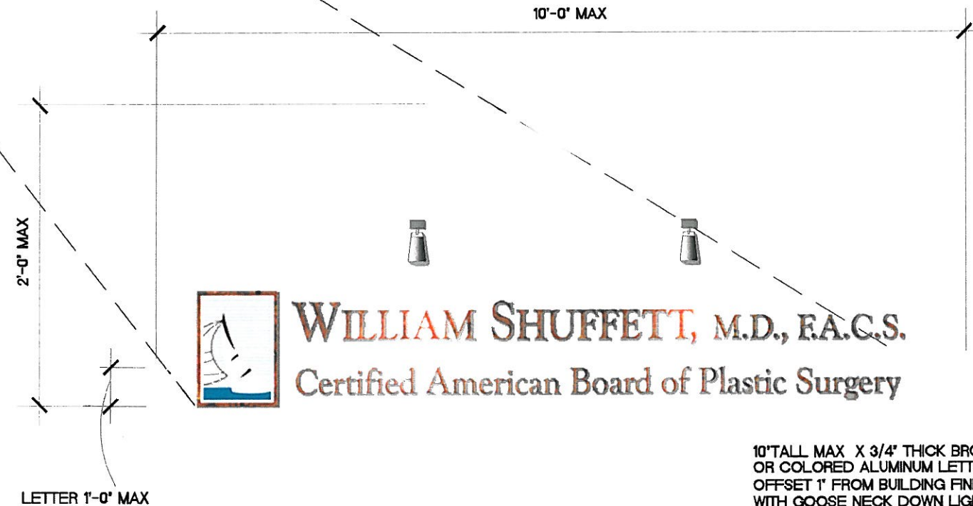
DIMENSIONAL LETTER SIGN FRONTAL VIEW SCALE: 1/2" = 1'-0"
