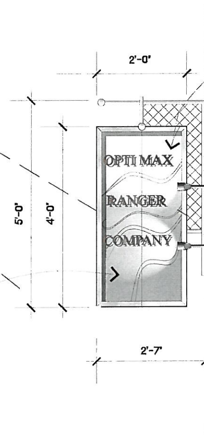
BLADE SIGN SIDE VIEW SCALE: 1/2" = 1'-0"
