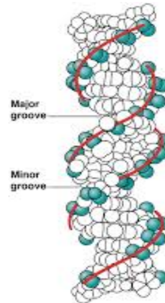
(a) B-DNA
