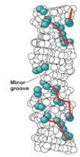
(b) Z-DNA
