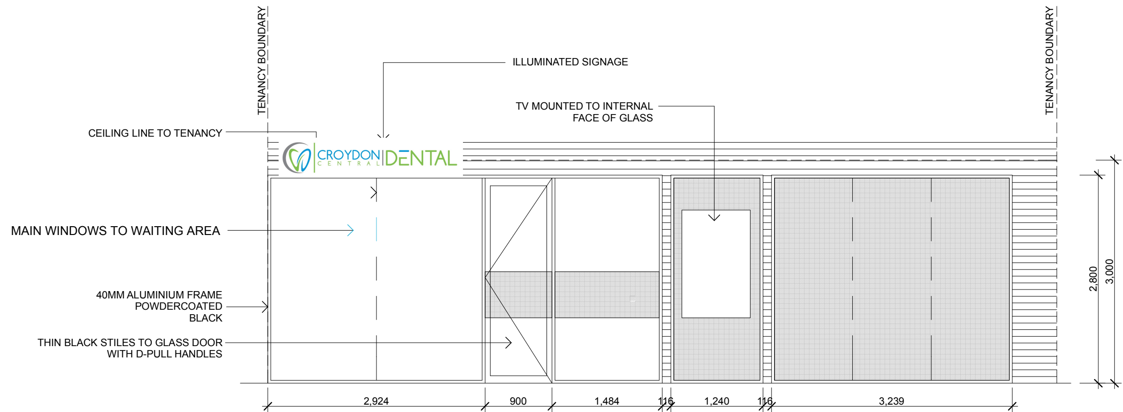
FACADE ELEVATION 1:50 @ A3
