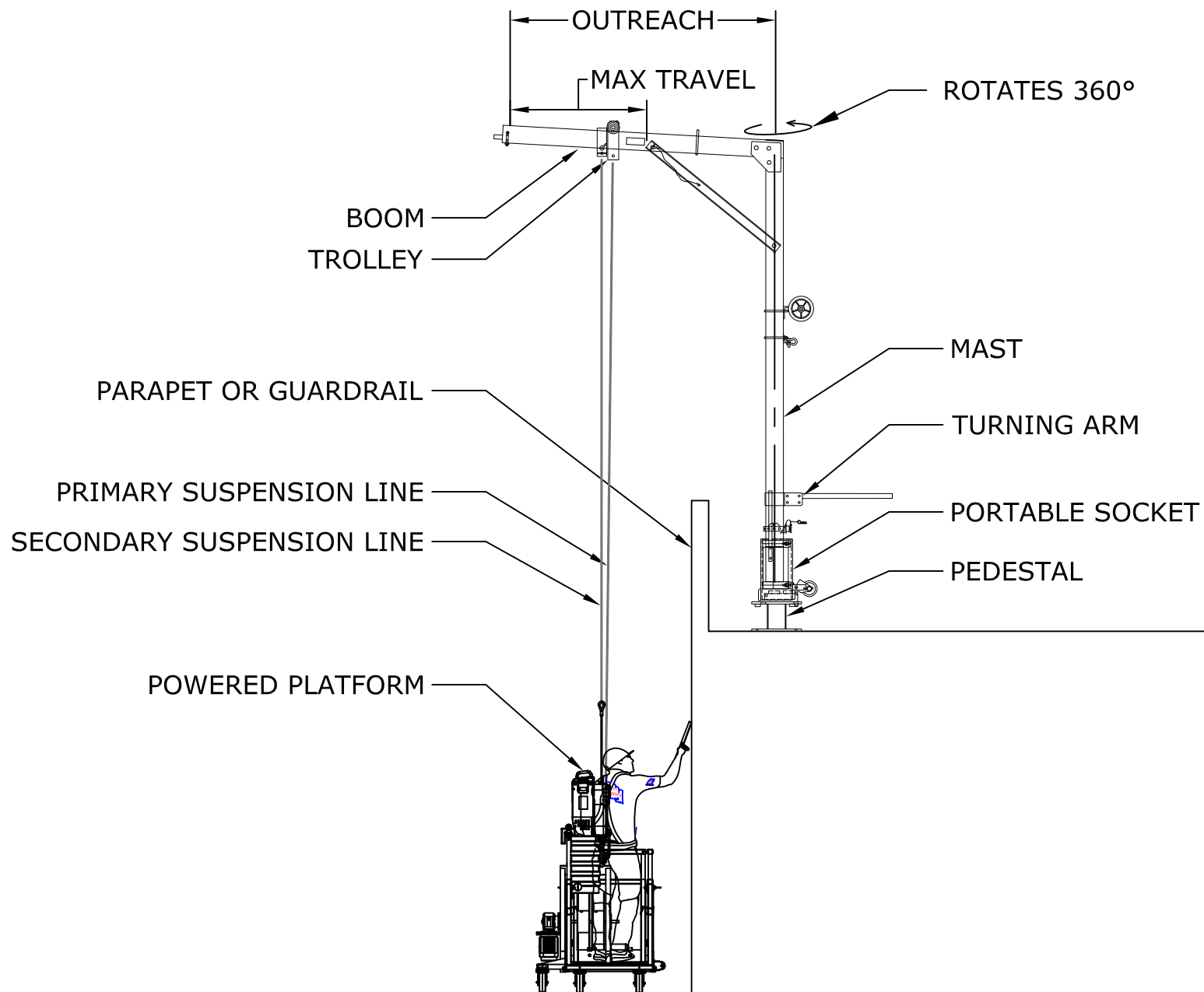
HIGH PROFILE BOTTOM ROTATING DAVIT IN USE
